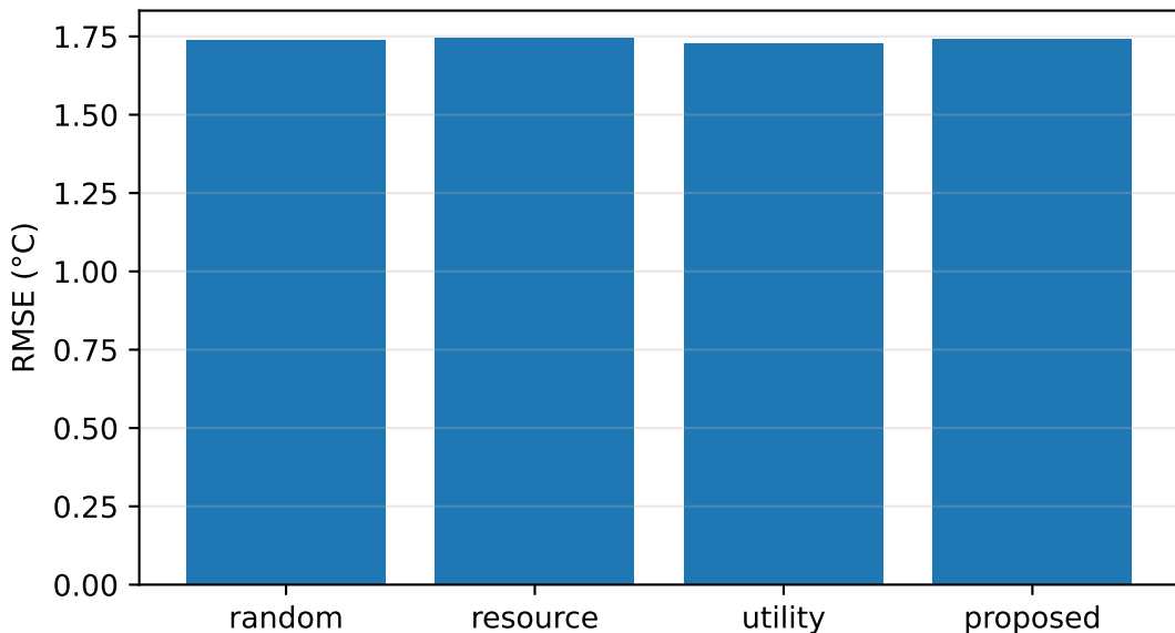
Intel Lab: RMSE ( ^{\circ}\text{C} ) at correlation 0.9
