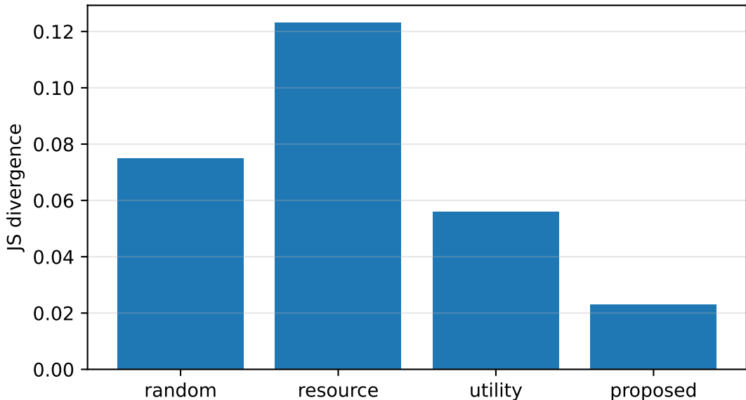
Intel Lab: JS divergence at correlation 0.9
