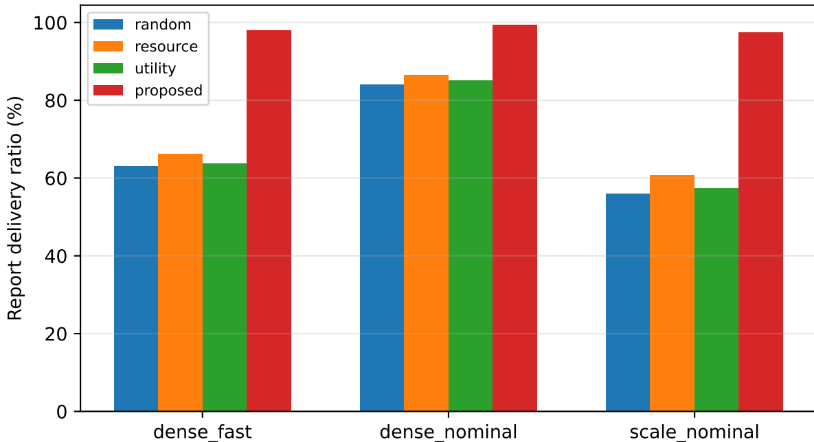
ns-3.47 LR-WPAN hop-equivalent validation
