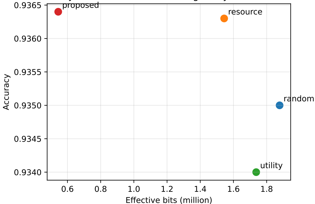
Synthetic correlated heterogeneity: trade-off
