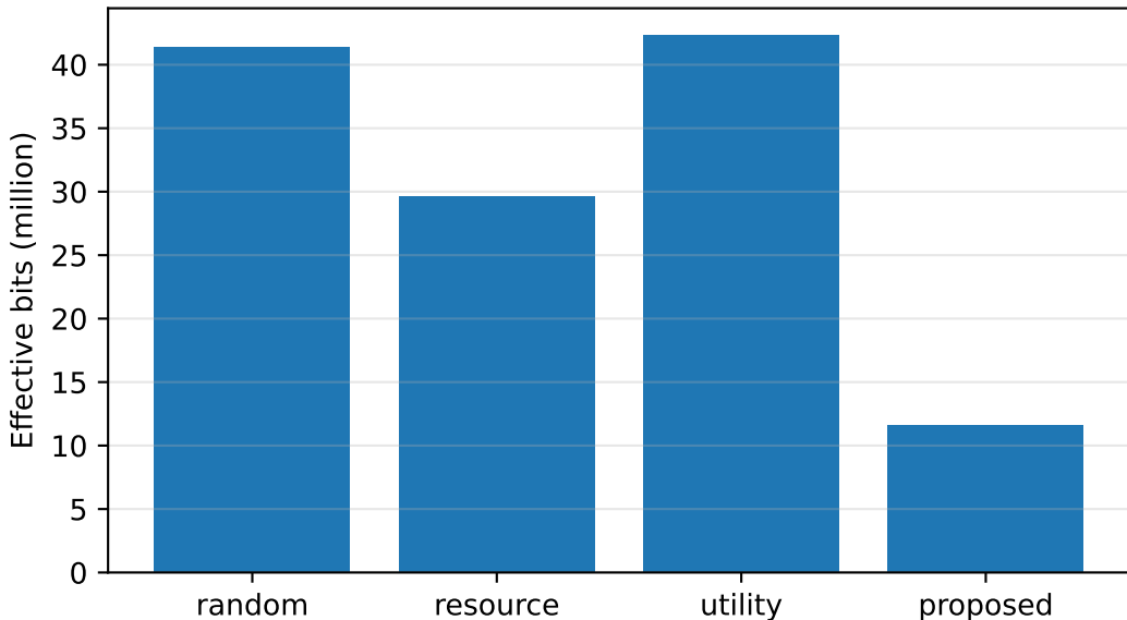
UCI HAR: Effective bits (million) at correlation 0.9
