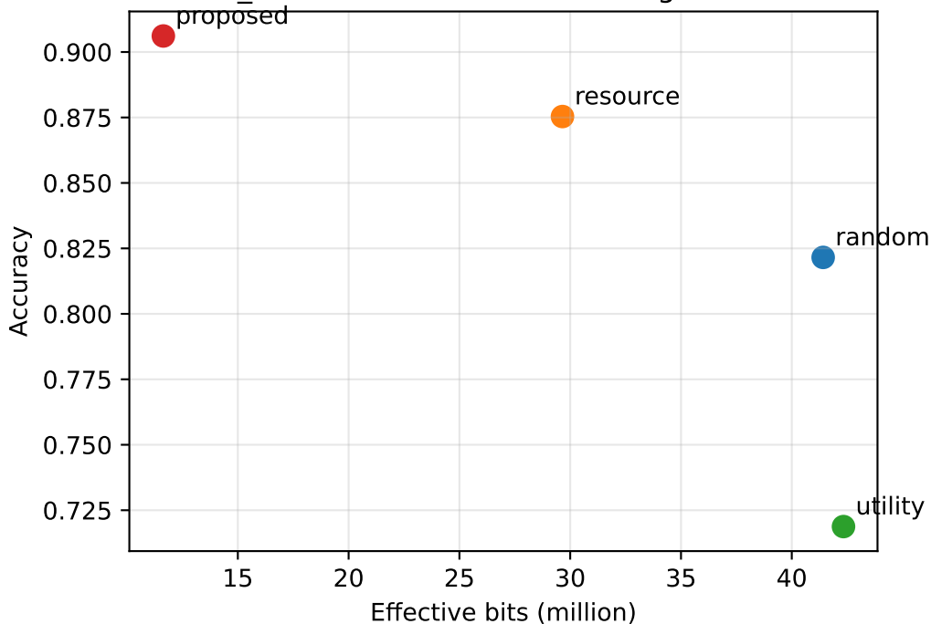
uci_har: communication-learning trade-off
