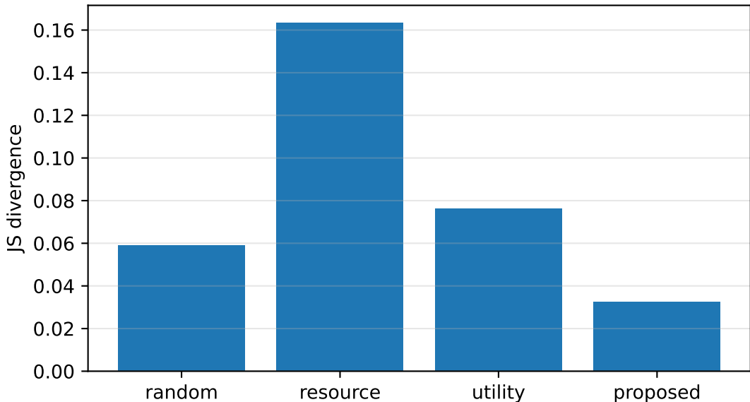
UCI HAR: JS divergence at correlation 0.9
