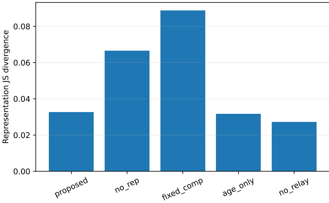
UCI HAR ablation: representation effect
