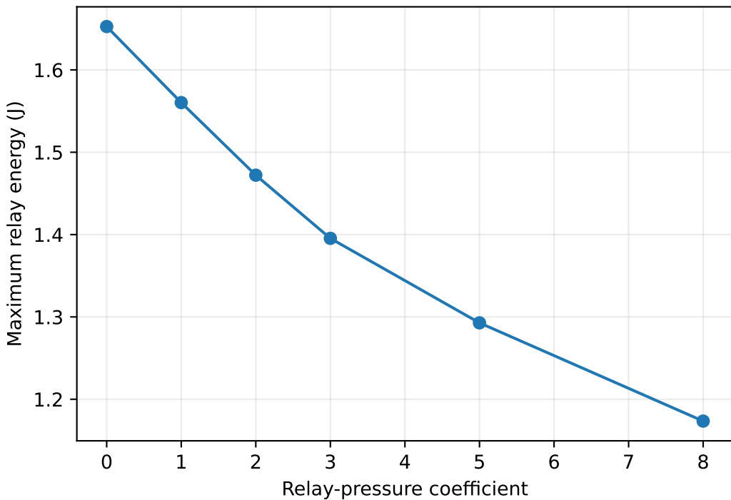
UCI HAR: relay-pressure sensitivity
