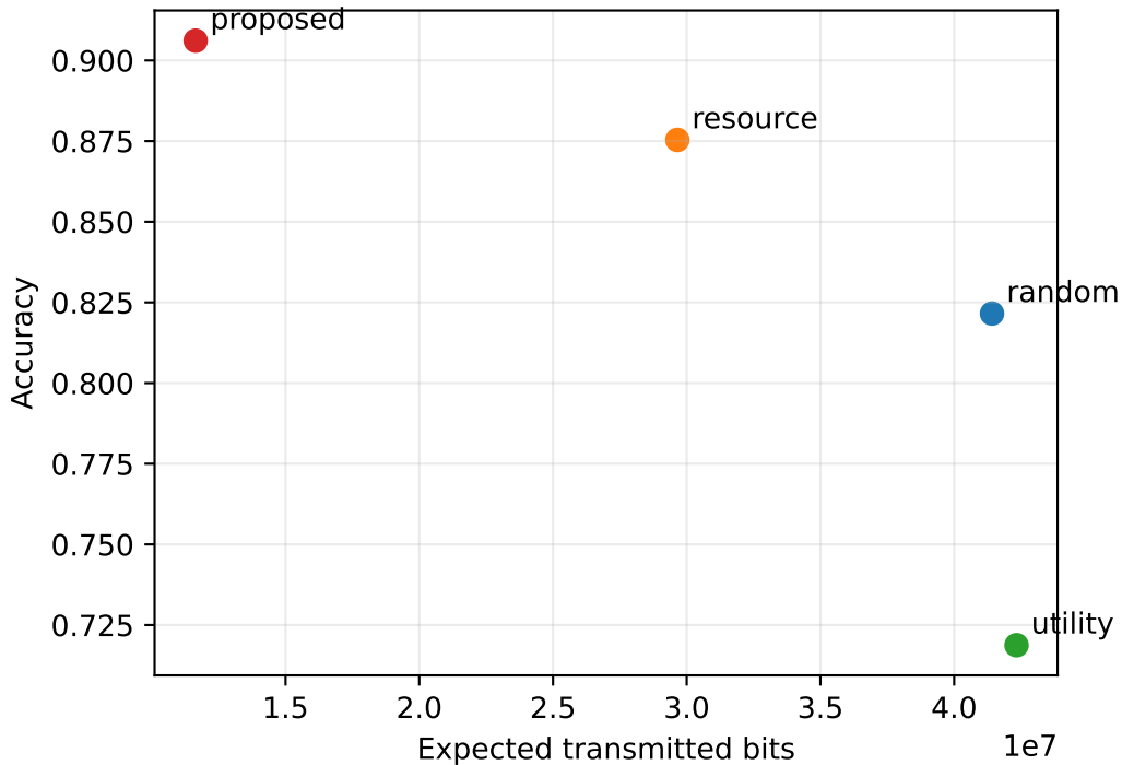
UCI HAR: communication-accuracy trade-off
