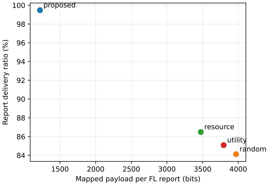
ns-3.47 LR-WPAN: dense nominal condition
