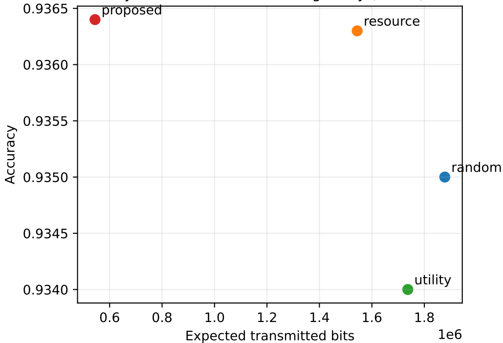
Synthetic correlated heterogeneity ( c=0.9 )
