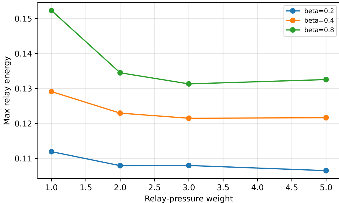
intel_lab: sensitivity of Max relay energy
