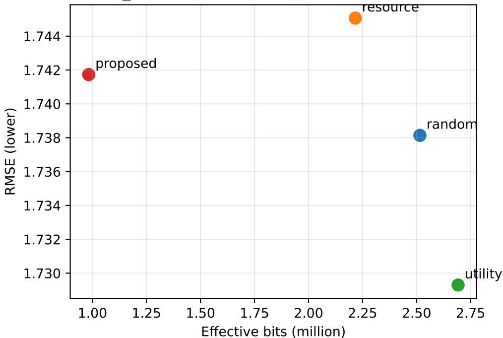
intel_lab: communication-performance frontier
