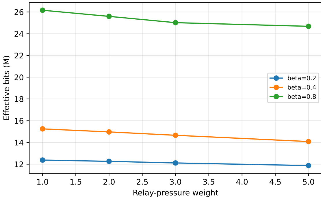
uci_har: sensitivity of Effective bits
