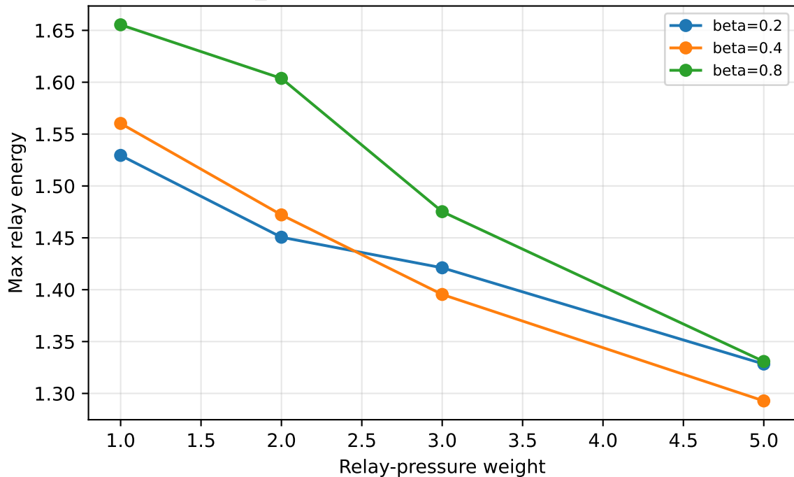
uci_har: sensitivity of Max relay energy
