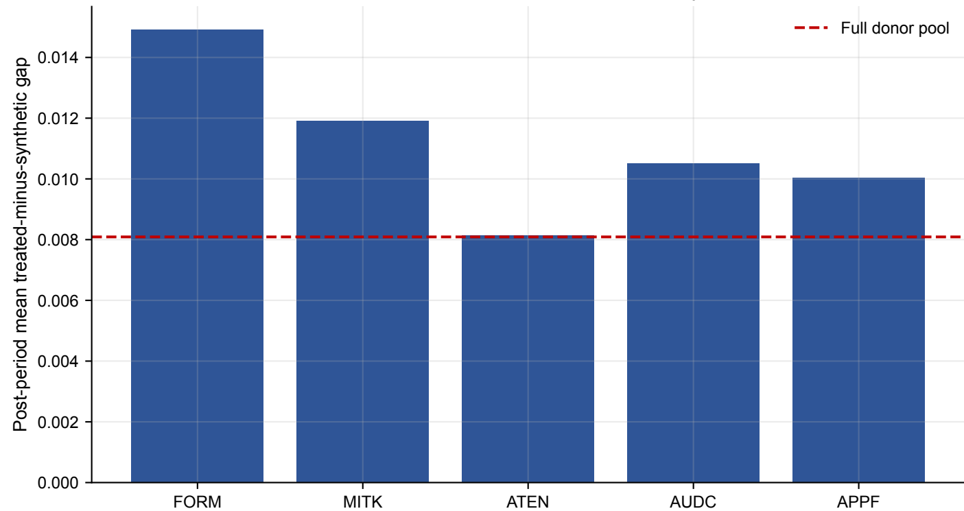
SCM Leave-One-Donor-Out Sensitivity
