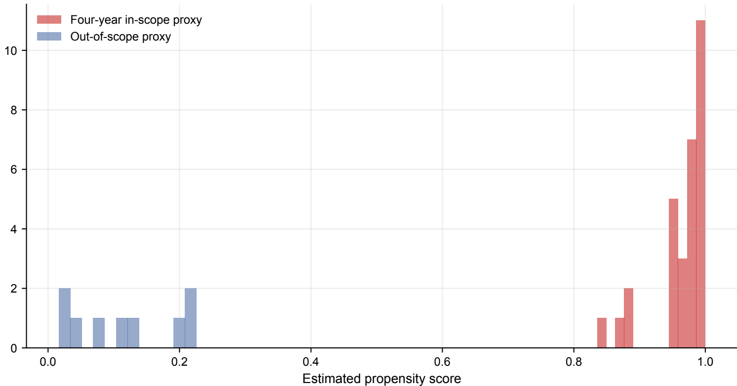
Common-Support Diagnostic before Overlap Weighting
