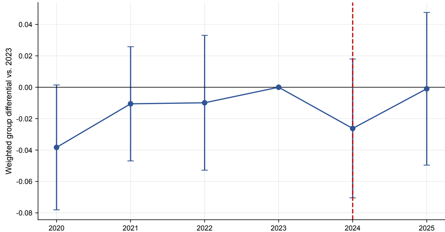
Overlap-Weighted DiD Parallel-Trends Diagnostic
