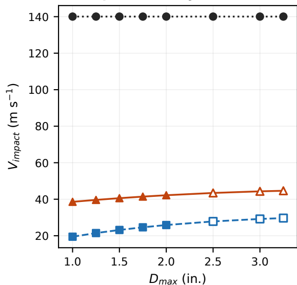
(a) Impact velocity vs. hail diameter
