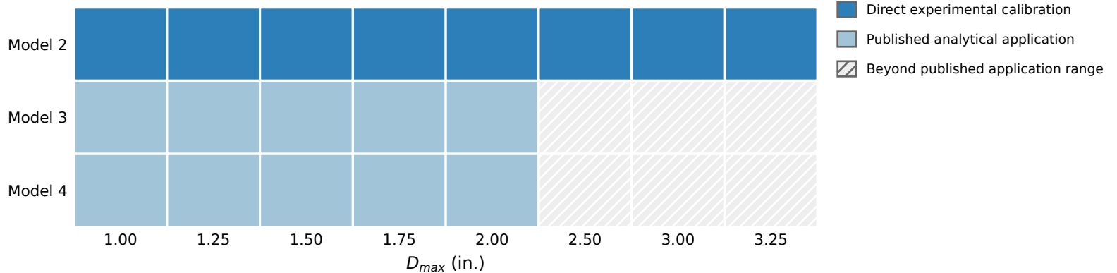
(c) Contact-model (Sun et al. 2015) evidence status
