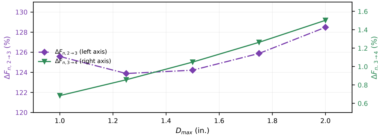
(b) Incremental change in peak normal force (applicable range only)
