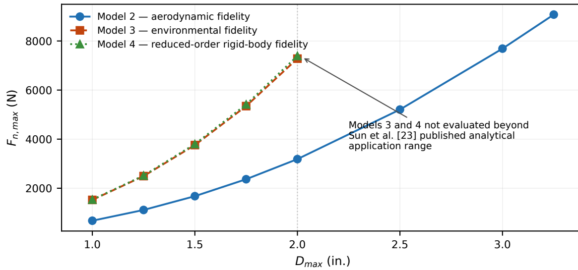
Figure 4. Effect of modeling fidelity on peak normal contact force (Models 2-4) (a) Peak normal contact force vs. hail diameter
