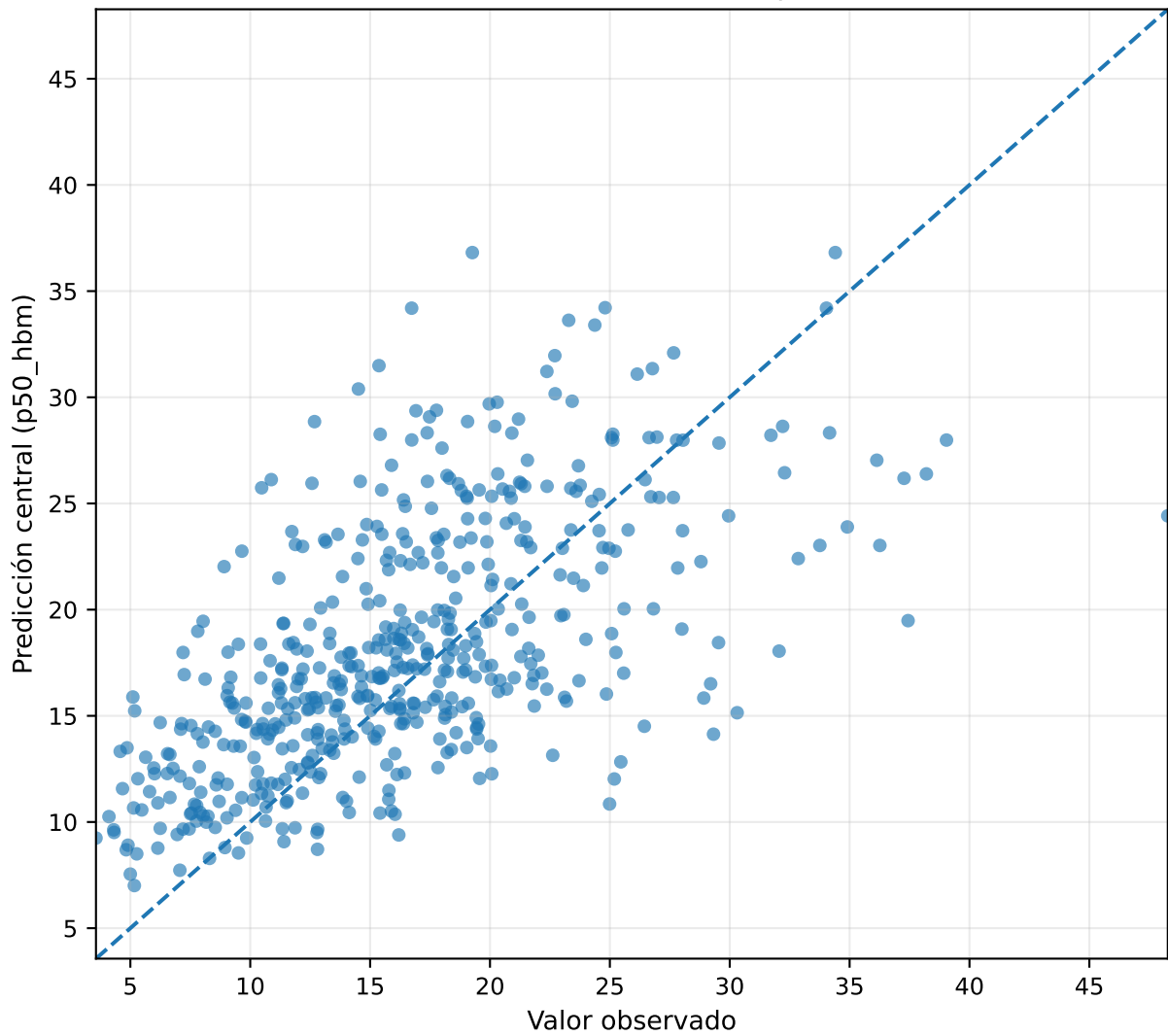
HBM PM2.5: observado vs. predicho
