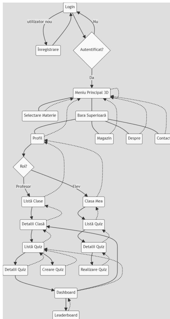
Figure 4.8: Diagrama de navigare a platformeiii
