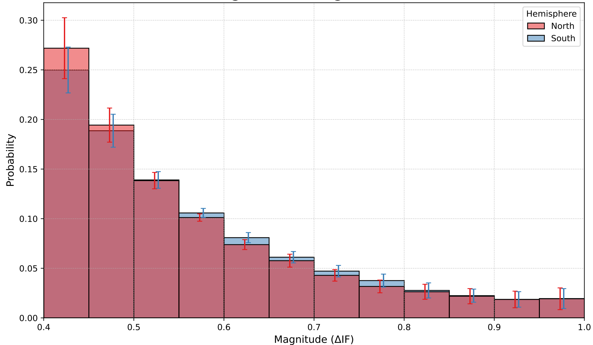
Distribution of glaciation magnitudes (N=1.11e+05)
