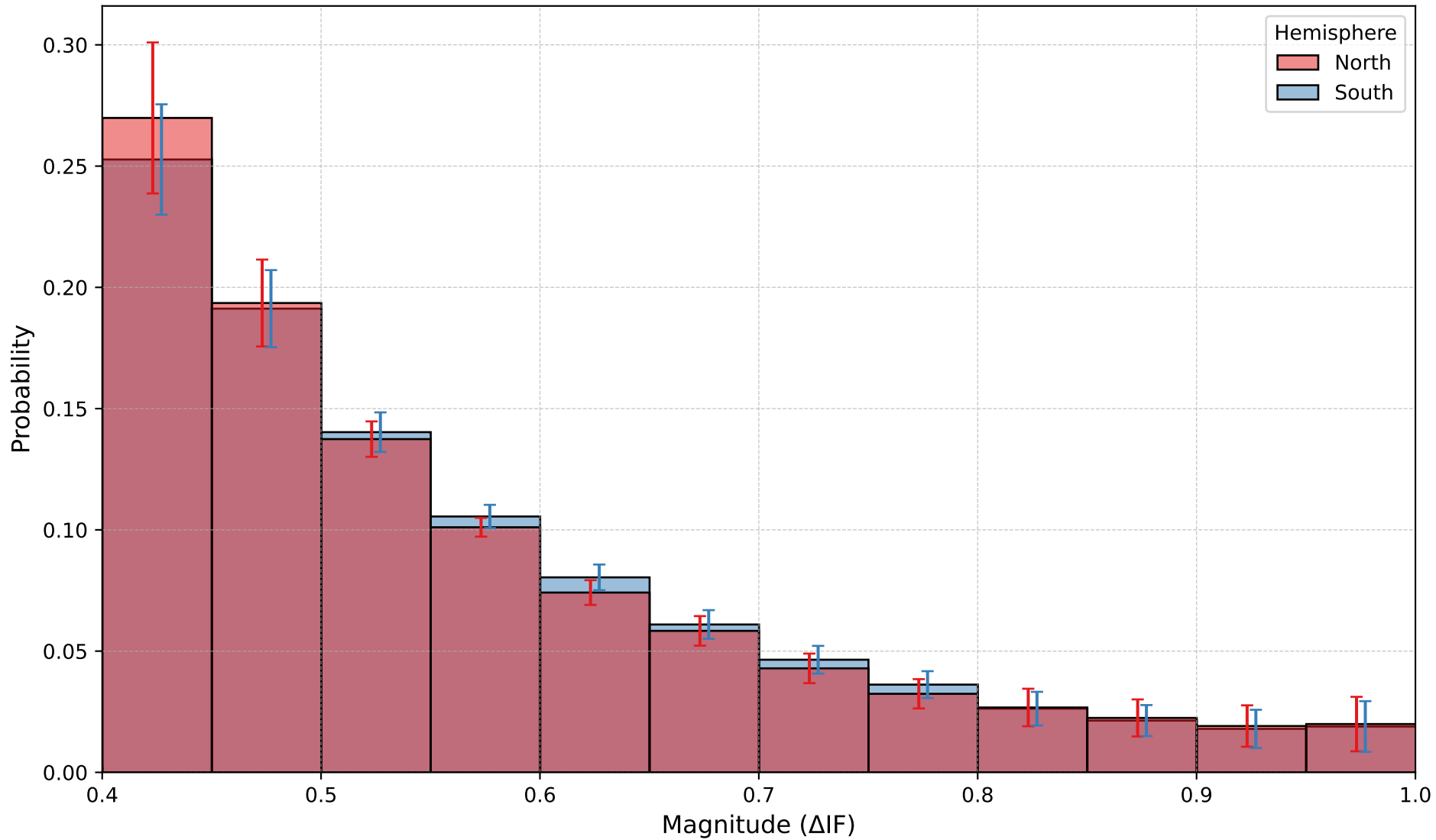
Distribution of glaciation magnitudes (N=1.01e+05)
