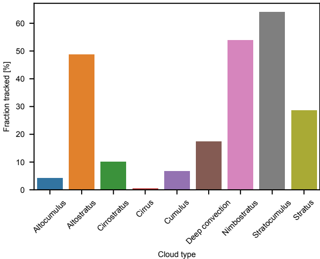
Faction of cloud area tracked for each cloud type
