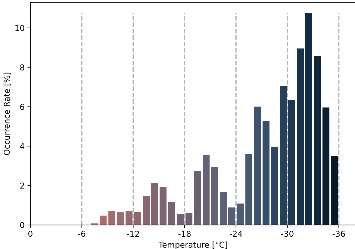
Occurrence Rate of Glaciation in 2010 in 1° Temperature Bins
