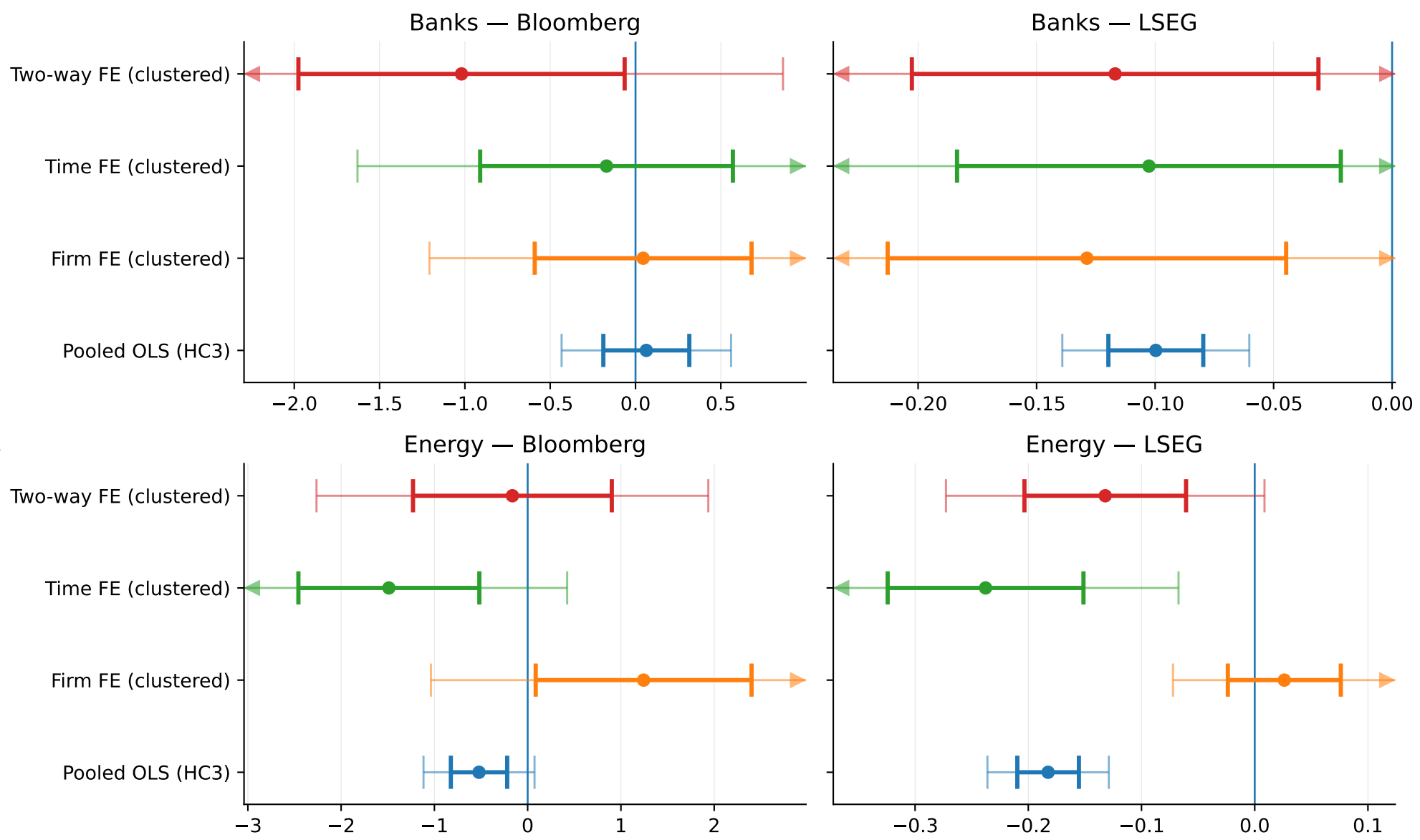
ESG coefficient estimate (dot) with 68% (thick) and 95% (thin) CIs
