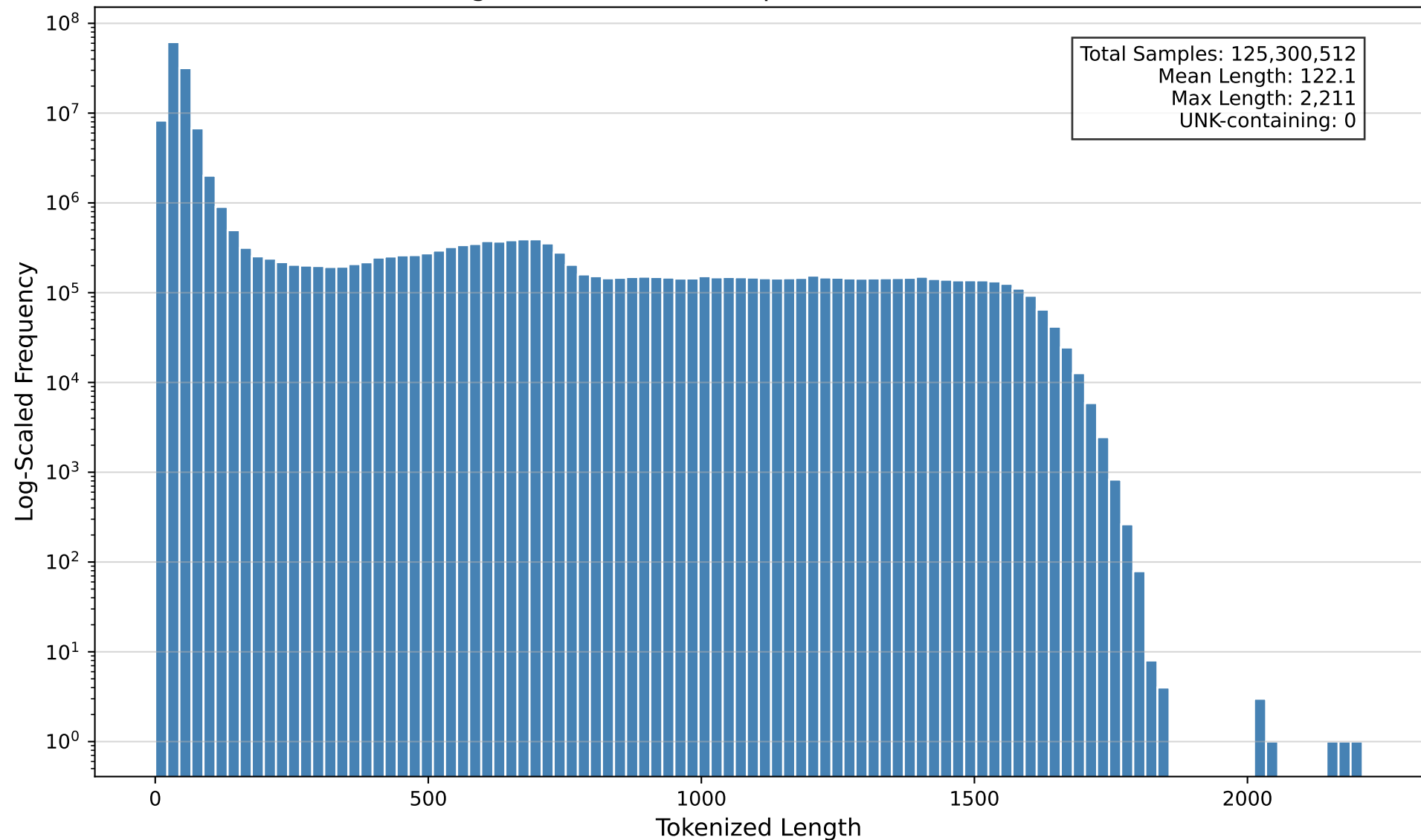
Token Length Distribution (DeepChem/ChemBERTa-77M-MTR)
