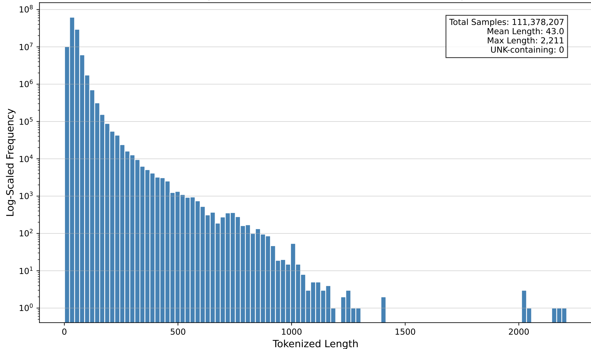
Token Length Distribution (ibm/MoLFormer-XL-both-10pct)
