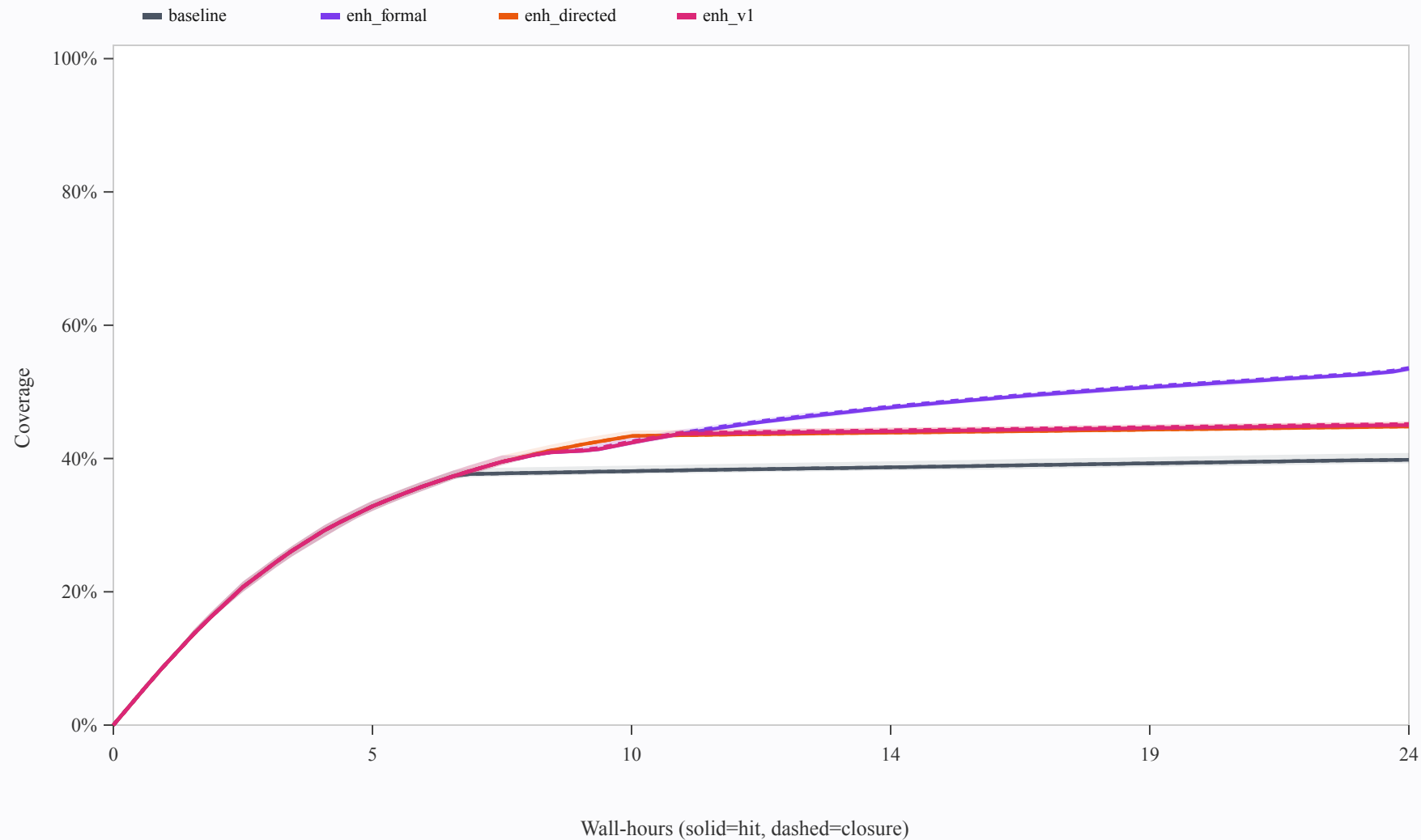
Coverage vs wall-hours — leftover-rich (5000 points, 10 seeds)
