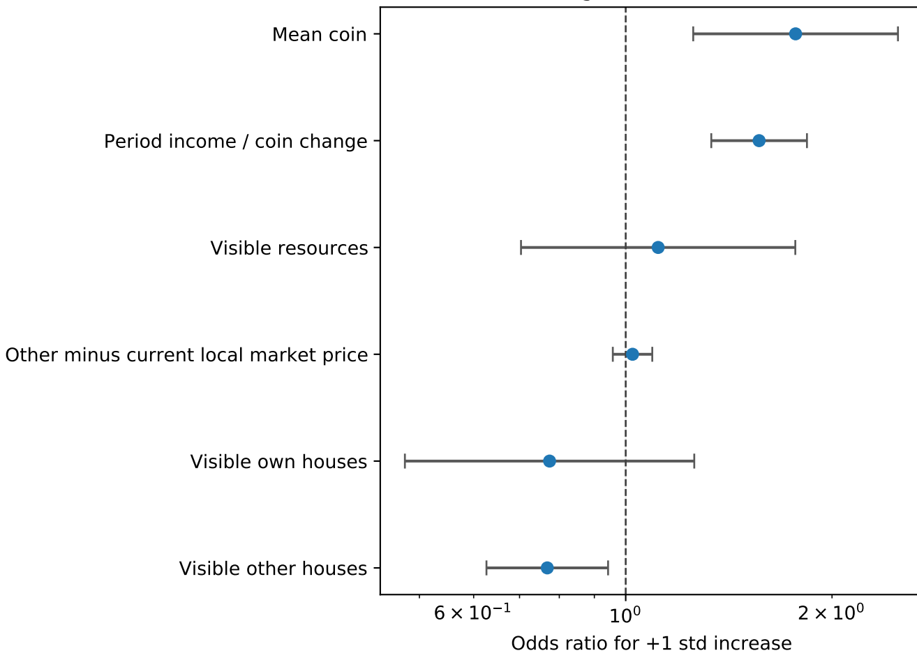
Variable Significance: Odds Ratios
