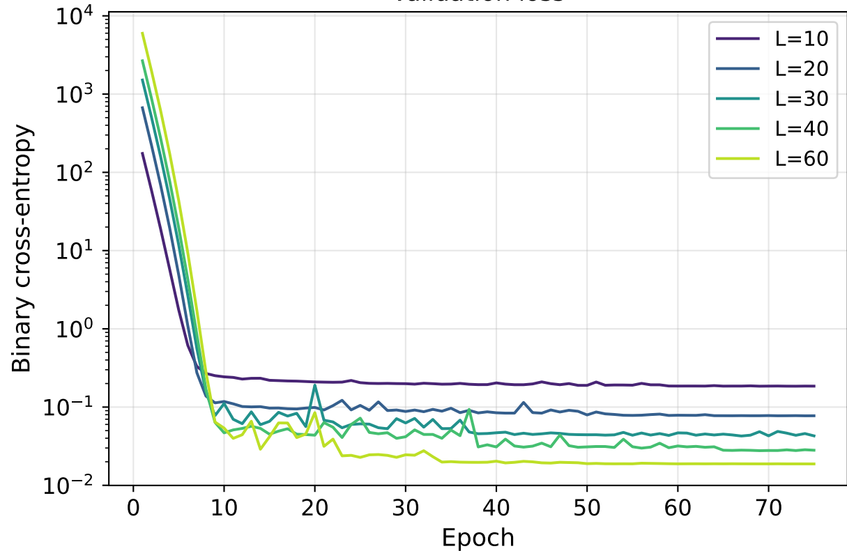
Validation loss
