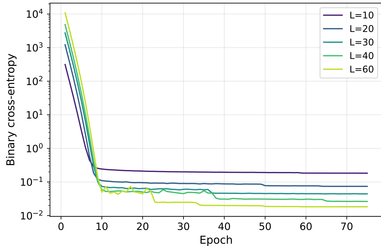
Train loss
