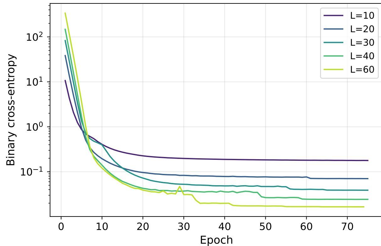
Train loss
