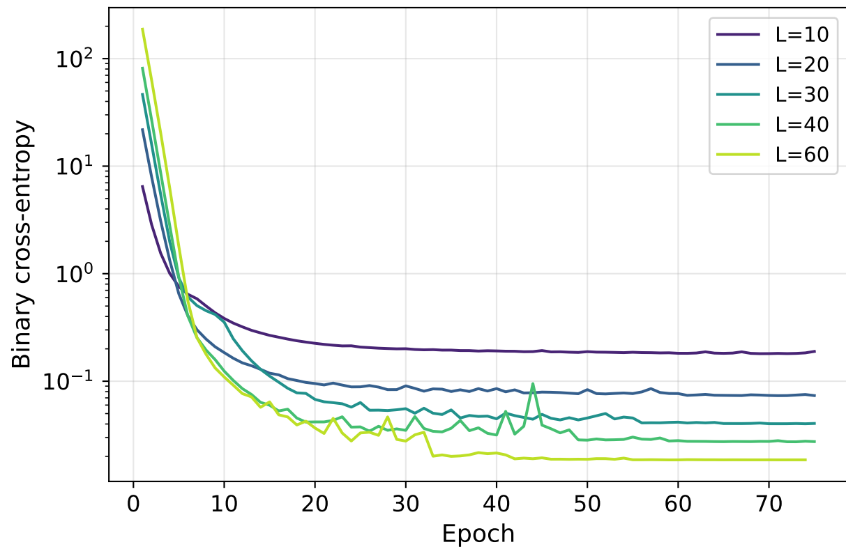
Validation loss
