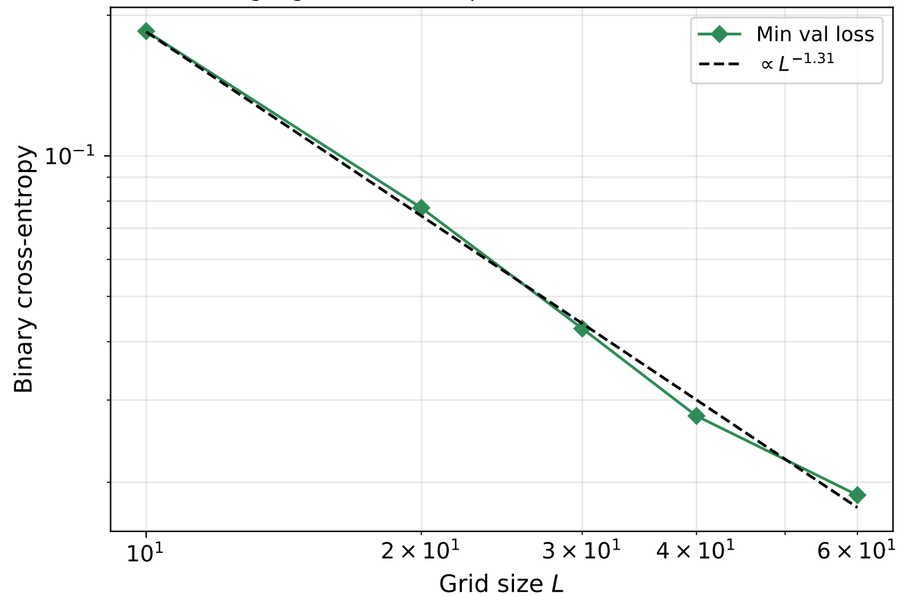
Log-log: Power-law Dependence of Validation Loss
