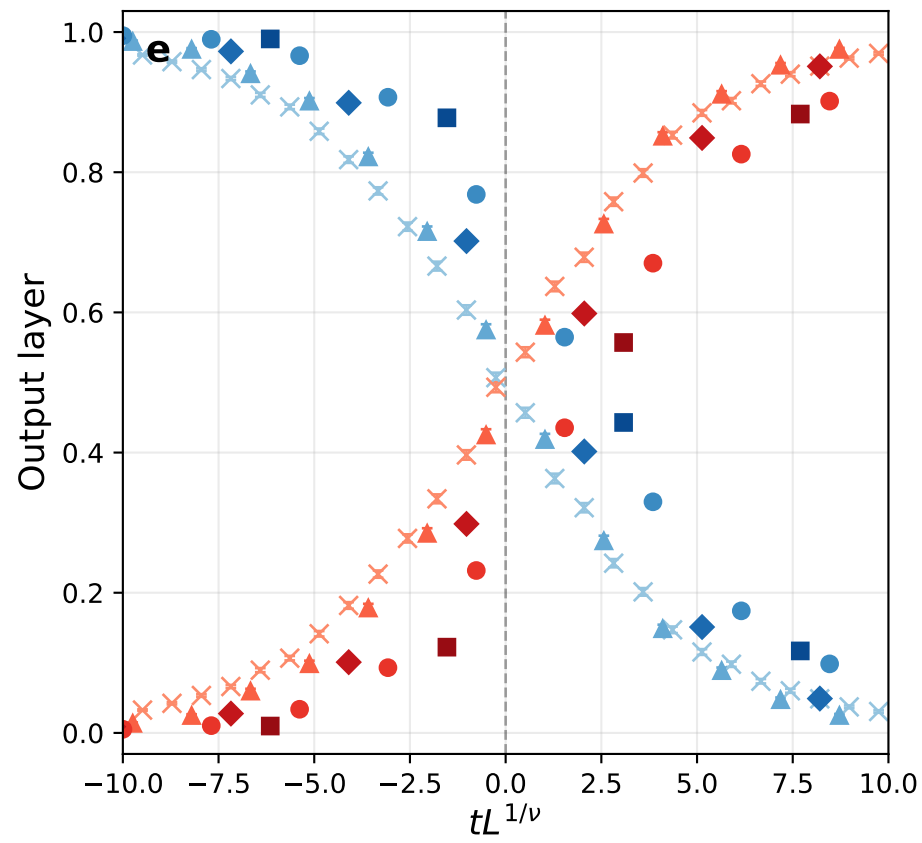
Finite-size scaling of CNN outputs — 2-D Ising model (square lattice)
