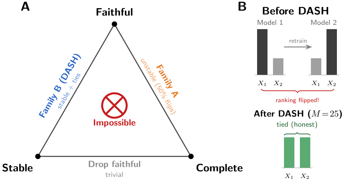
Figure 1: The Attribution Impossibility. No importance ranking can be simultaneously faithful, stable, and complete under symmetry. Faithful, Stable, Complete: Pick Two . Family \mathcal{A} (single-model) is faithful and complete but rankings flip up to 50% of the time. Family \mathcal{B} (stable projection: DASH for features, G -invariant for circuits) is stable with zero unfaithfulness but reports ties for symmetric elements (sacrificing completeness). No third option exists.
