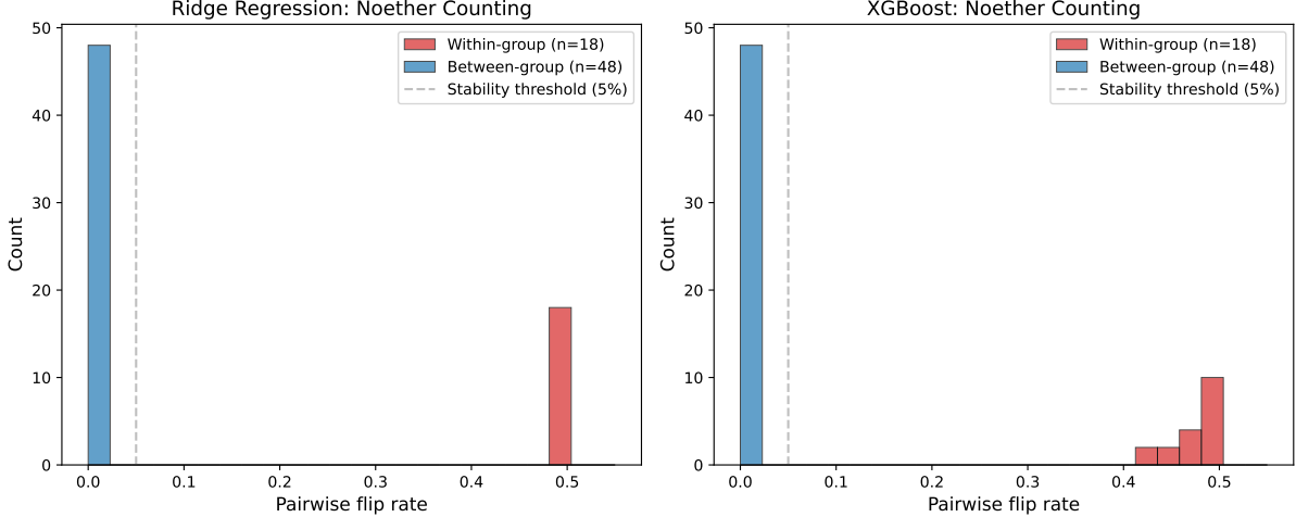
Figure 4: Invariance counting experiment (cf. Noether’s theorem). Pairwise flip rates for 66 feature pairs across 200 models, showing a sharp bimodal separation: within-group pairs (red) cluster at \sim 50\% (coin flip), while between-group pairs (blue) cluster at \sim 0\% (perfectly stable). The bimodal gap of 47 percentage points confirms that exactly \binom{g}{2} = 3 independent group-level ranking facts are stably answerable.
