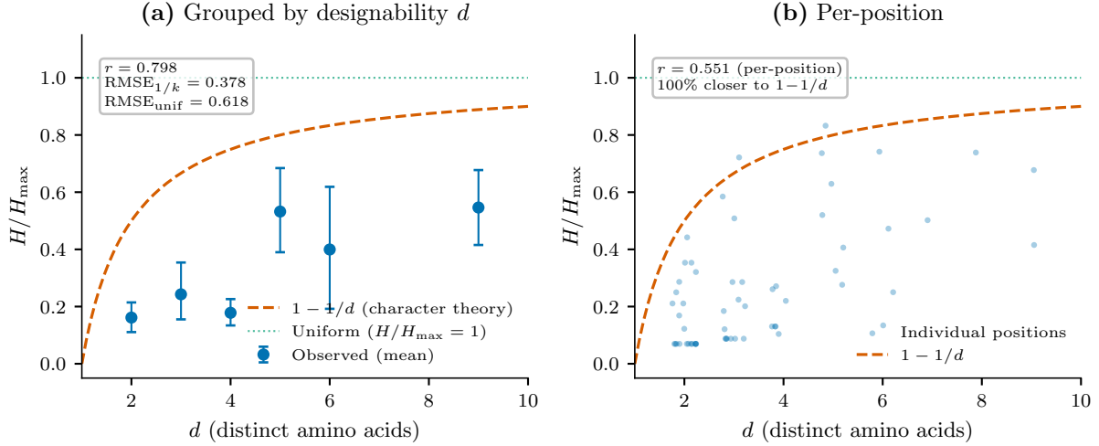
Figure 3: Protein sequence diversity at aligned cytochrome c positions vs. the character-theory prediction (d - 1)/d . All 59 variable positions lie closer to the character-theory curve than to uniform, with systematic undershoot attributable to purifying selection. Pearson r = 0.798 , Spearman \rho = 0.881 .
