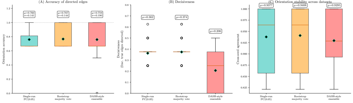
Figure 4: DASH-style ensemble averaging transferred to causal discovery (Asia network, 100 seeds, 50 bootstrap resamples). The ensemble reduces the orientation flip rate by 4\times while trading off decisiveness, confirming the trilemma tradeoff in a new domain.
