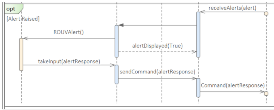
Figure 8: Section of RCU Sequences sequence diagram, showing alert catching behaviour on receipt of alert
