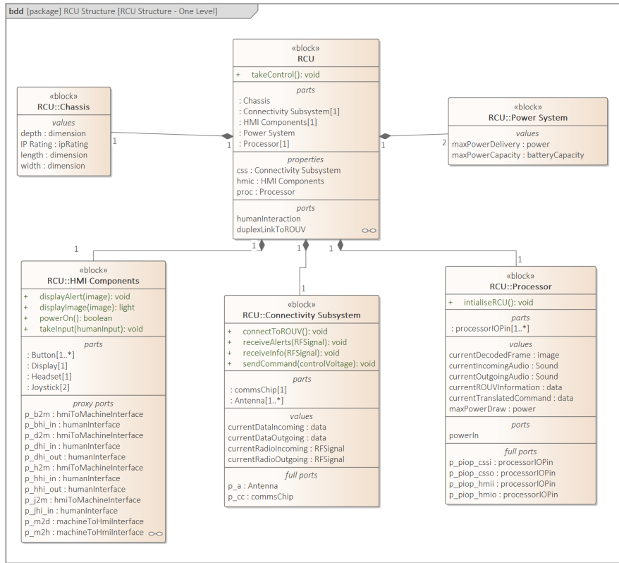
Figure 4: Top Level Block Definition Diagram
