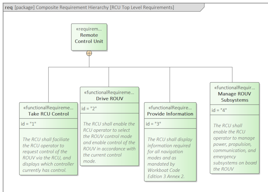
Figure 2: RCU Top Level Requirements
