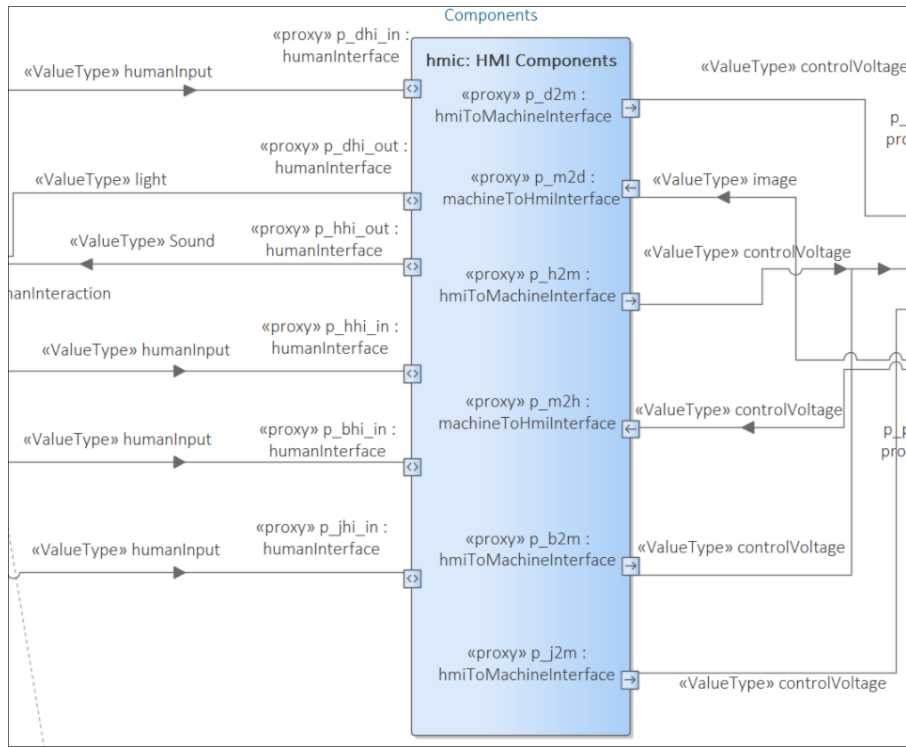
Figure 5: Section of RCU IBD, showing HMI item type conversion
