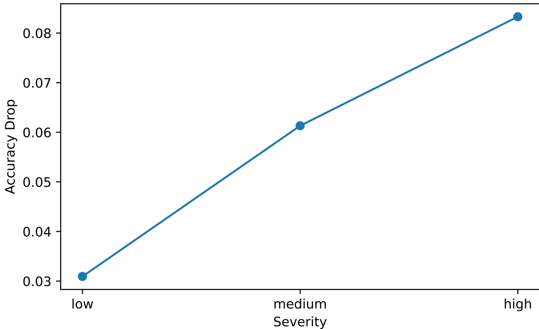
hhar CNN1D noise robustness
