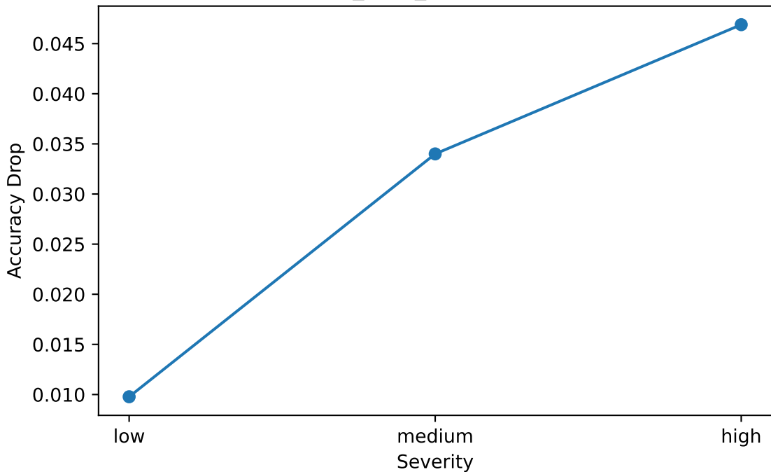
hhar Improved_GNN_LSTM noise robustness
