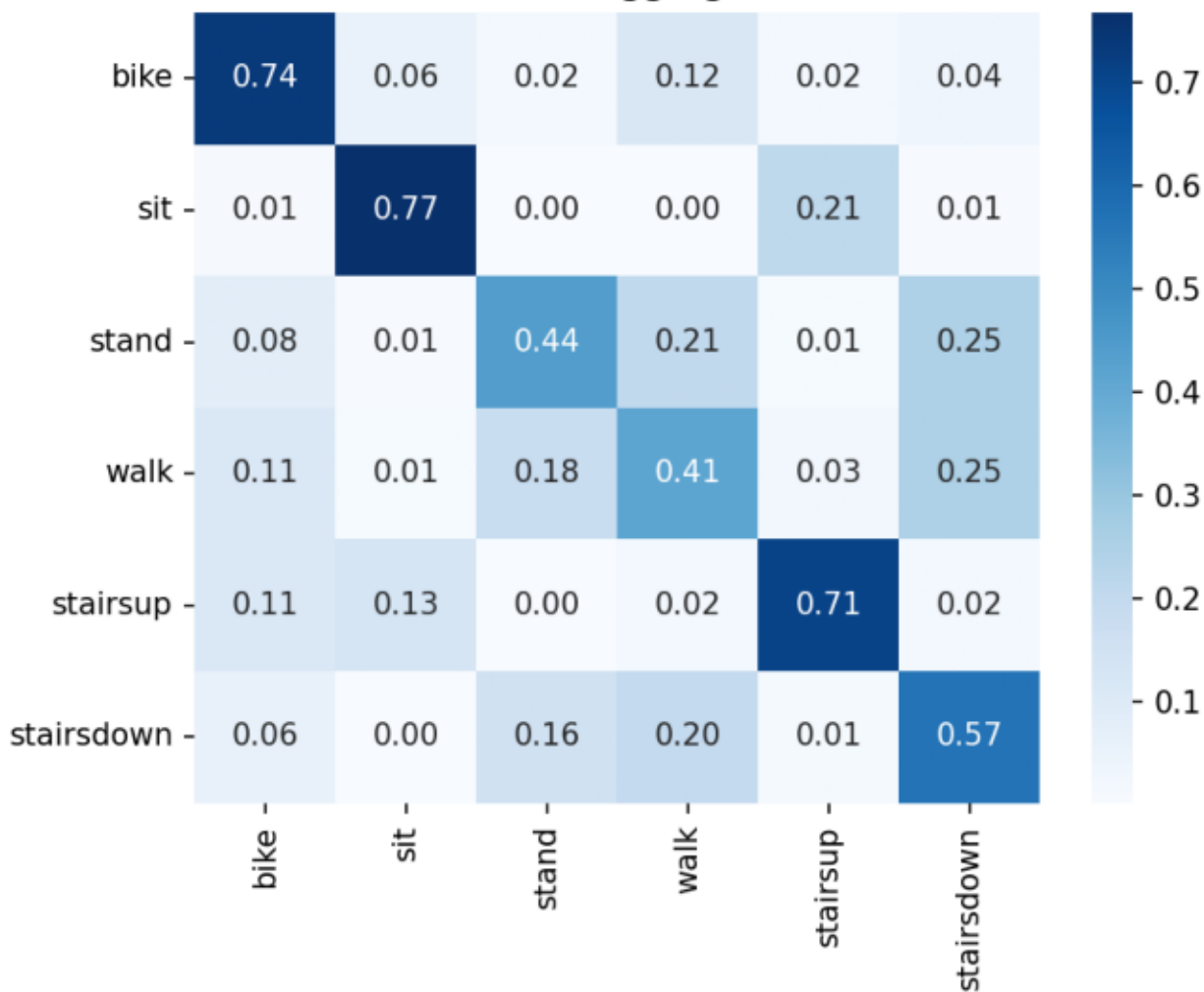
hhar CNN1D aggregated CM
