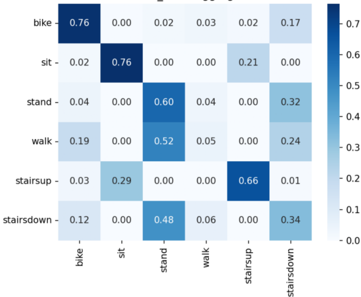
hhar Flatten_LSTM aggregated CM
