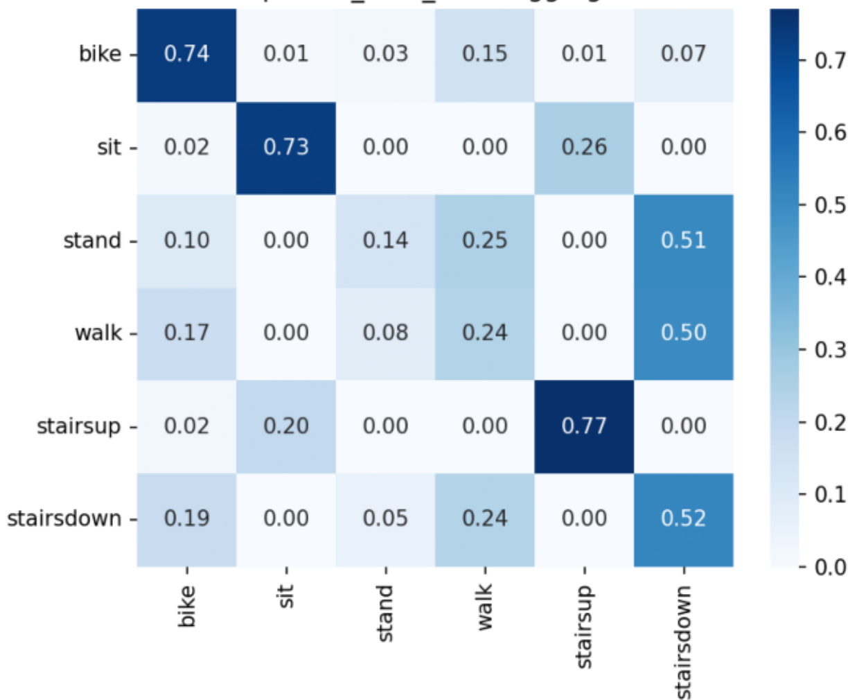
hhar Improved_GNN_LSTM aggregated CM
