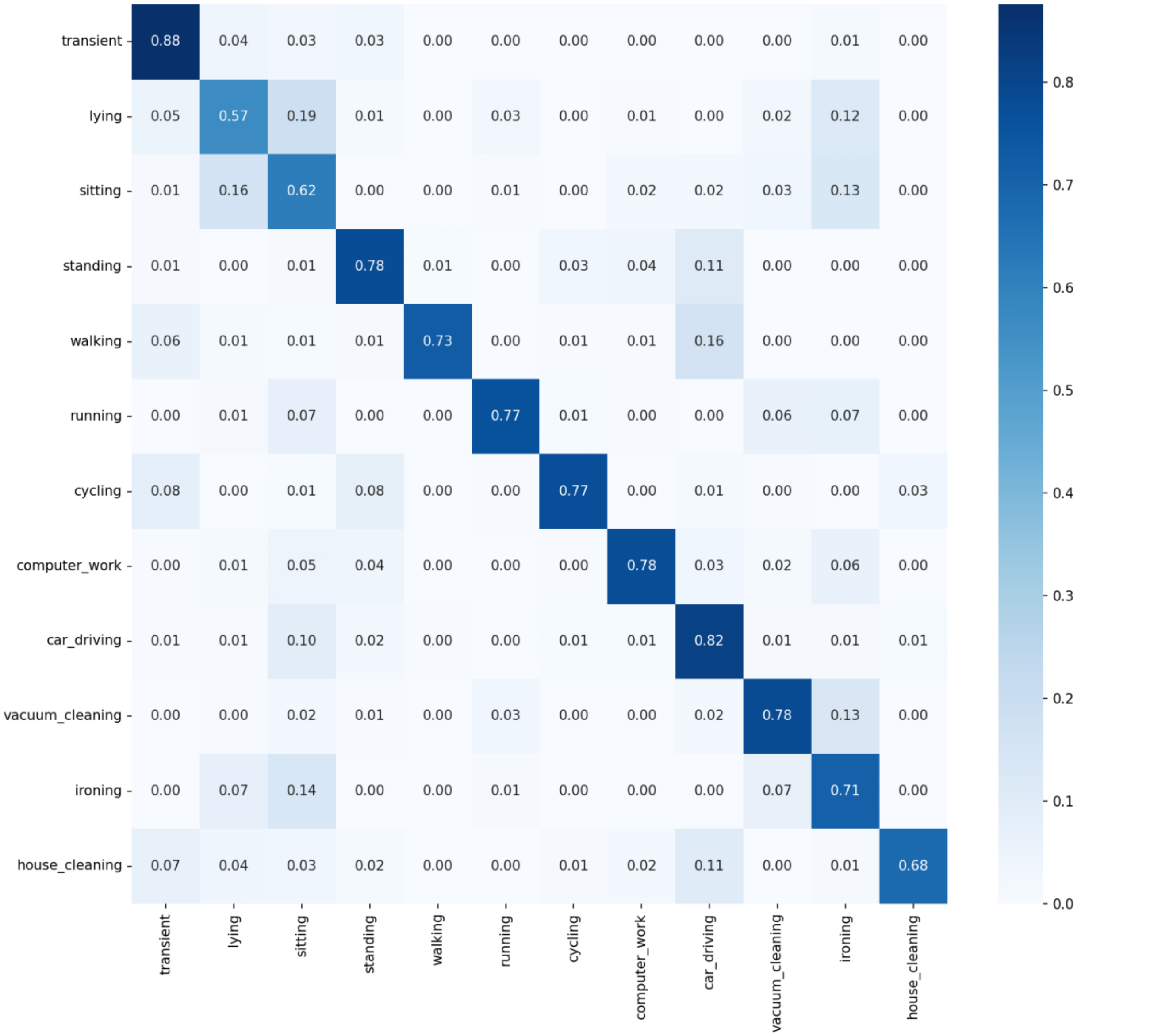
pamap2 CNN1D aggregated CM
