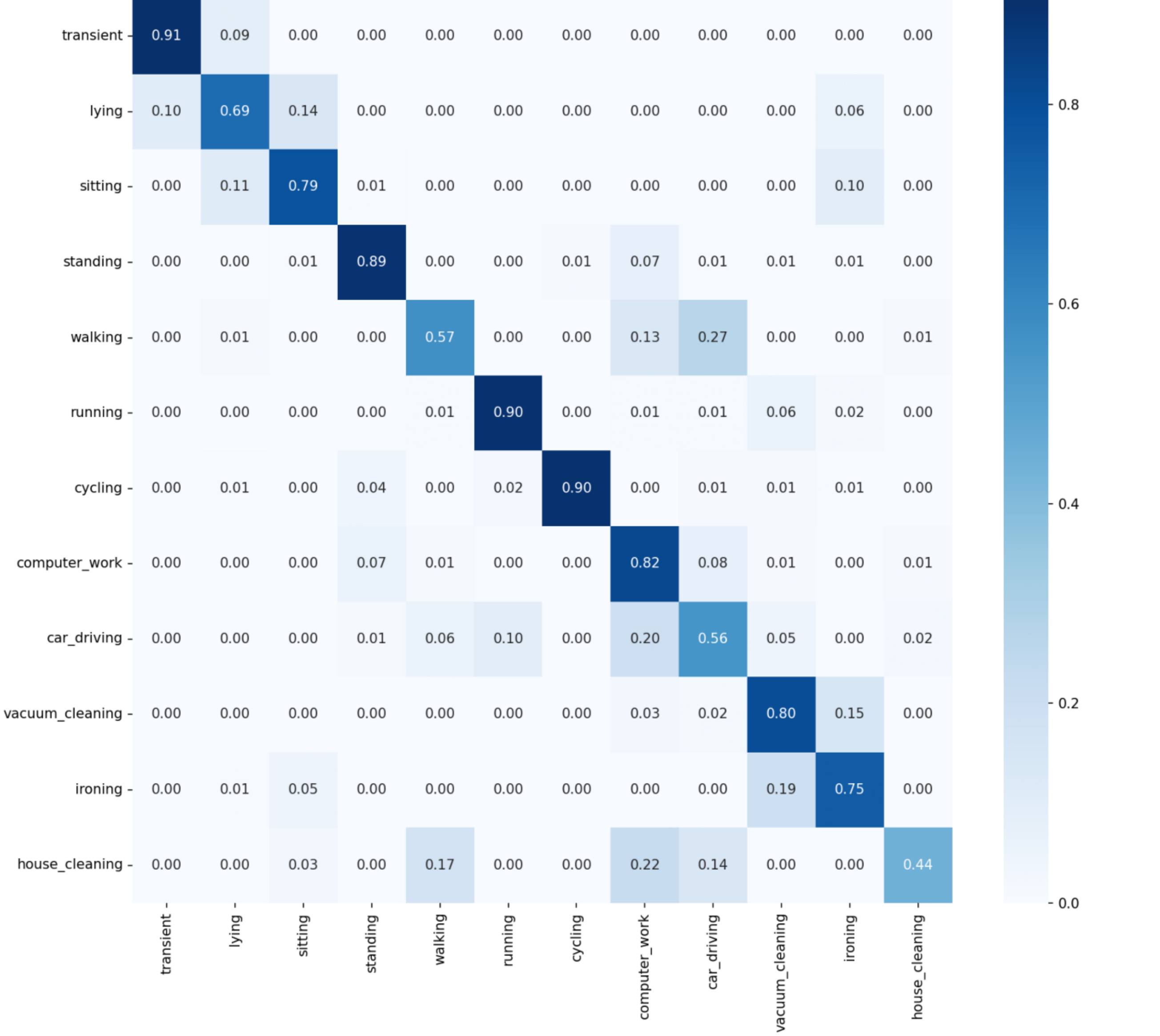
pamap2 Flatten_LSTM aggregated CM
