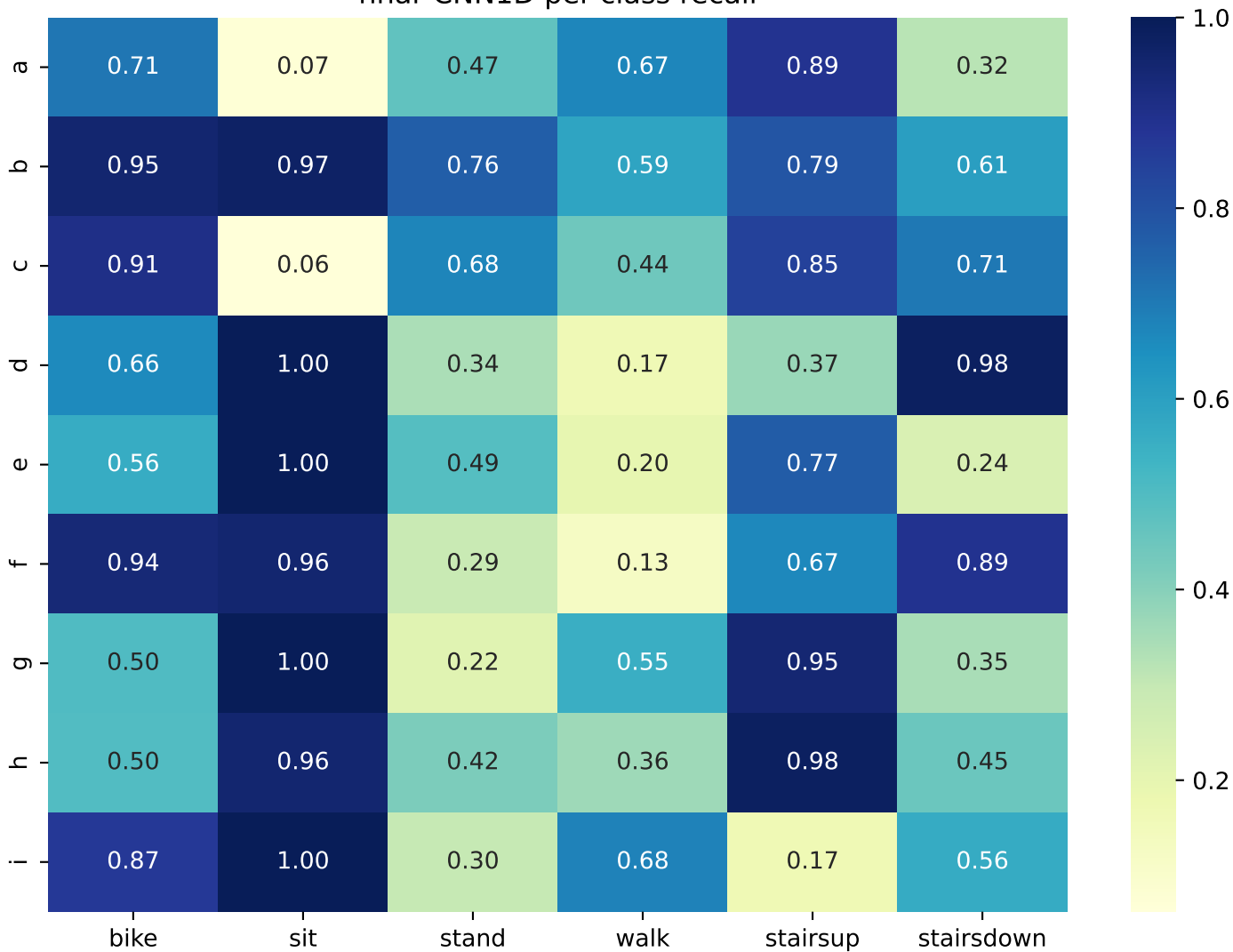
hhar CNN1D per-class recall
