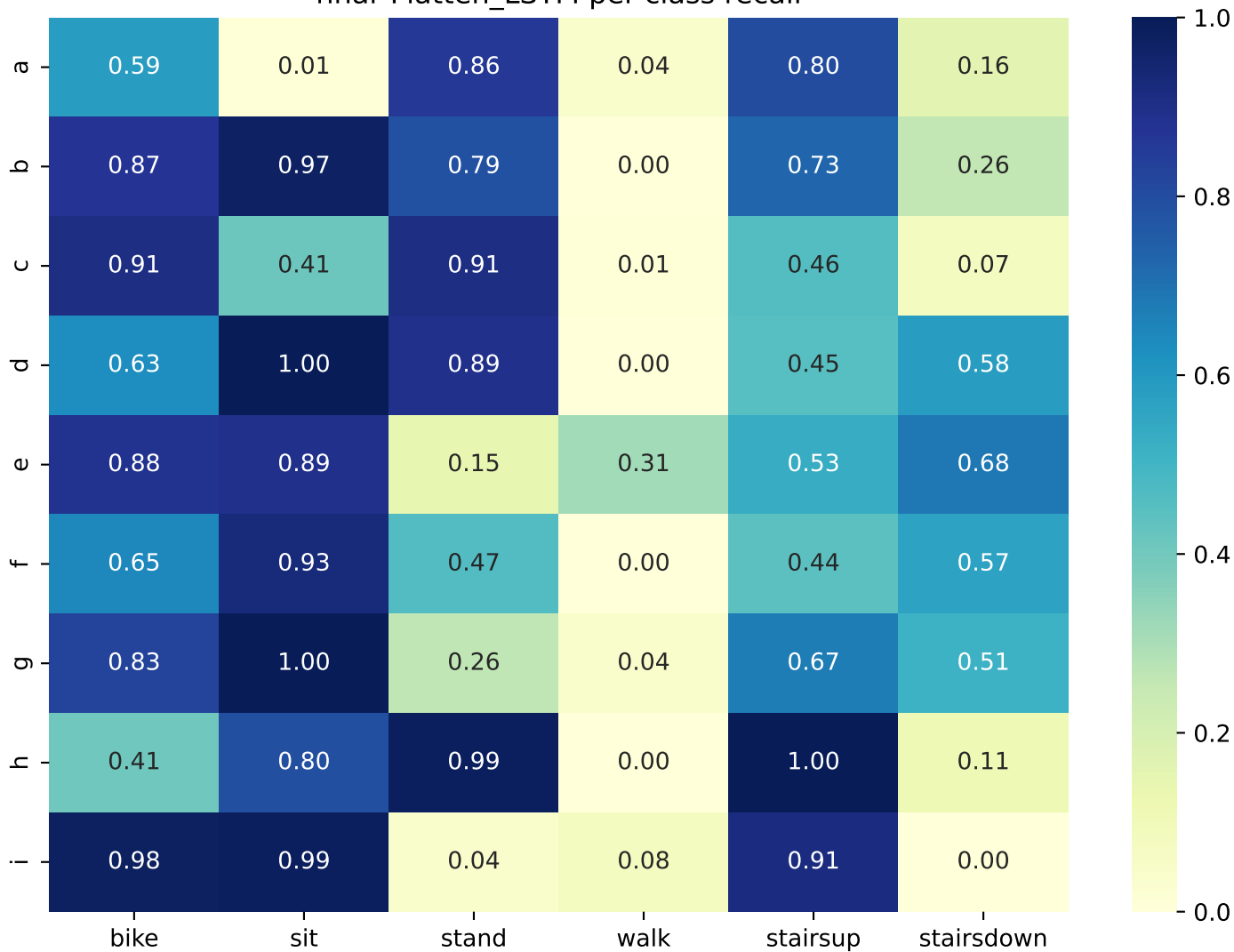
hhar Flatten_LSTM per-class recall
