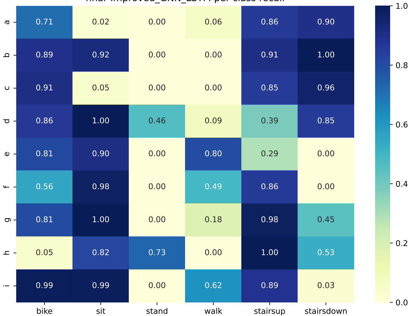
hhar Improved_GNN_LSTM per-class recall
